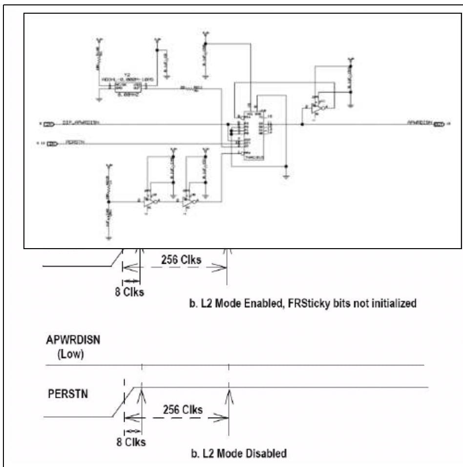
Figure 2.3 APWRDIS# Timing
