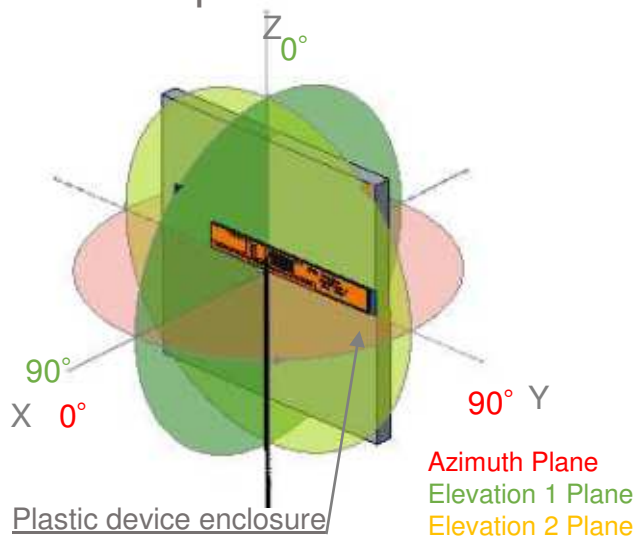
Test setup
