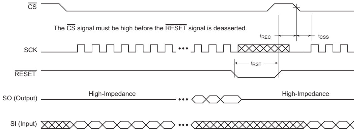
Figure 58. Reset Timing
