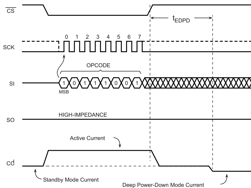
Figure 19. Deep Power-Down
