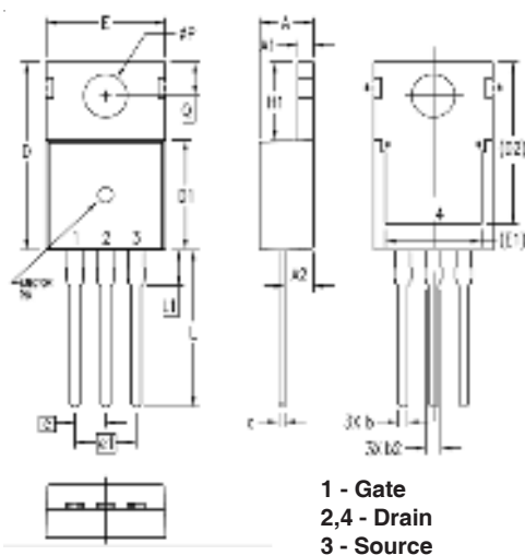
TO-220 Outline
