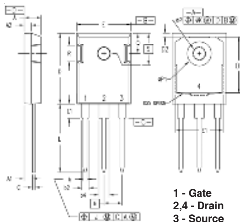
TO-247 Outline
