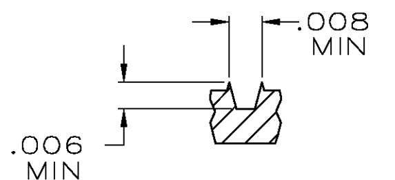
SERRATION DETAIL SCALE 20:1
