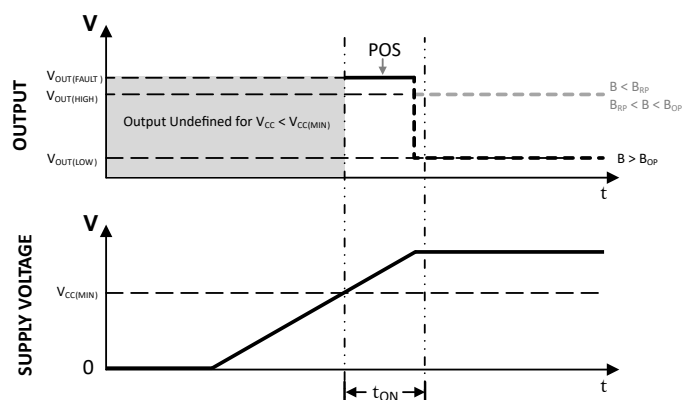
Figure 4: Power-On Sequence
