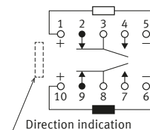
2 coil latching ( Reset )
