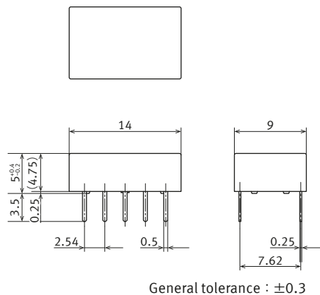
External dimensions PC board terminal ( standard )
