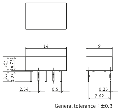
PC board terminal ( self-clinching terminal )
