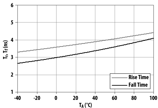
Figure 9. Typical rise and fall time versus temperature at 3.3 V supply voltage.
