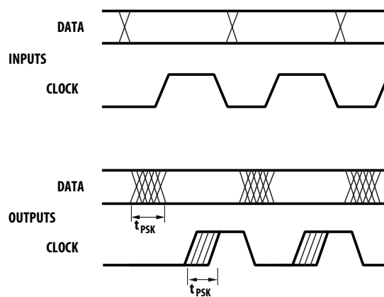
Figure 14. Parallel data transmission example
