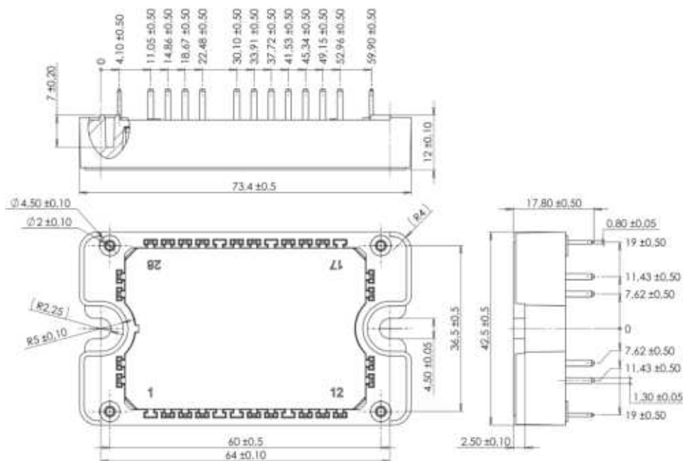
Figure 20 • Package Outline
