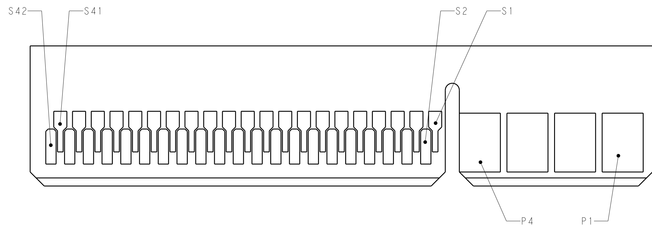
RECOMMENDED MATING BOARD EDGE CONFIGURATION (SECONDARY SIDE SHOWN)
