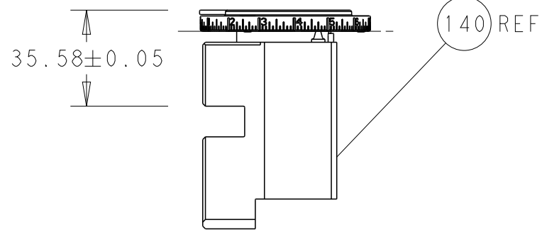
RAM SET-UP
