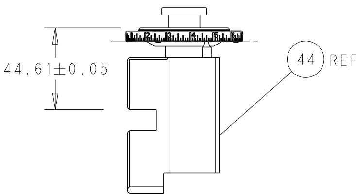
RAM SET-UP
