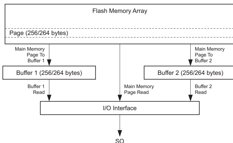
Figure 34. Block Diagram
