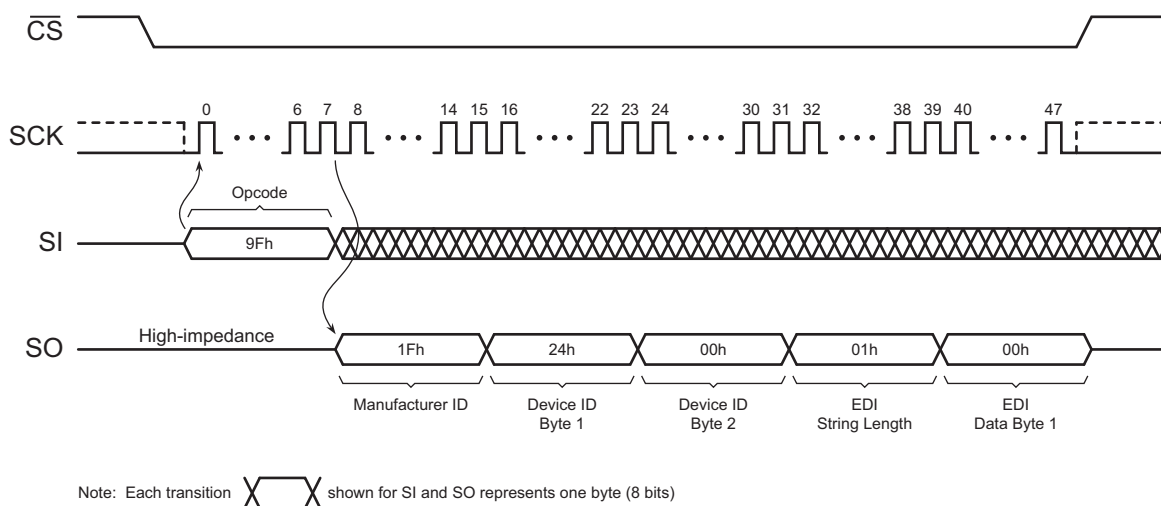
Figure 48. Manufacturer and Device Read Timing (Opcode 9Fh)
