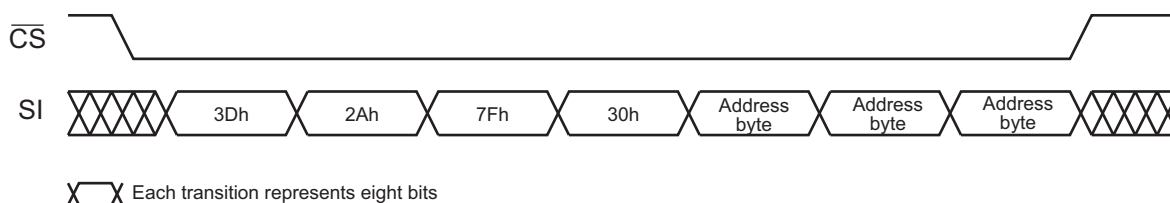
Figure 11. Sector Lockdown
