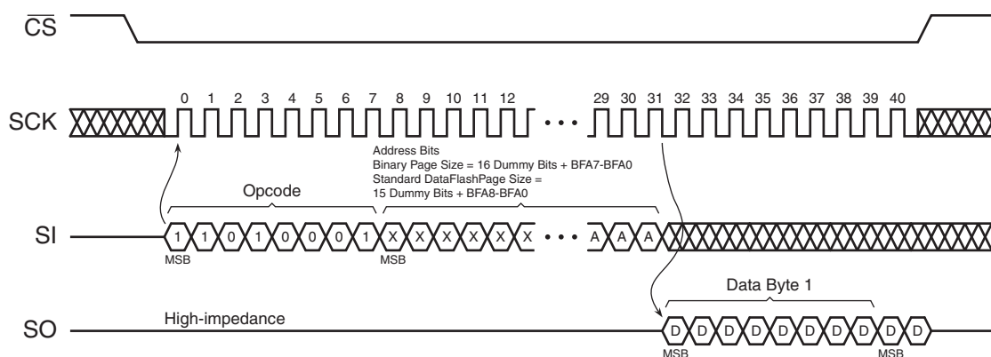
Figure 43. Buffer Read – Low Frequency Timing (Opcode D1h or D3h)
