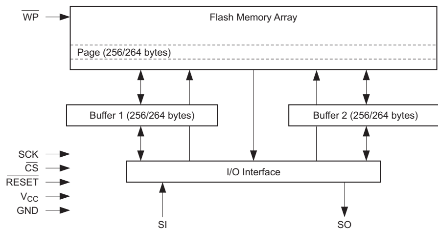
Figure 2. Block Diagram
