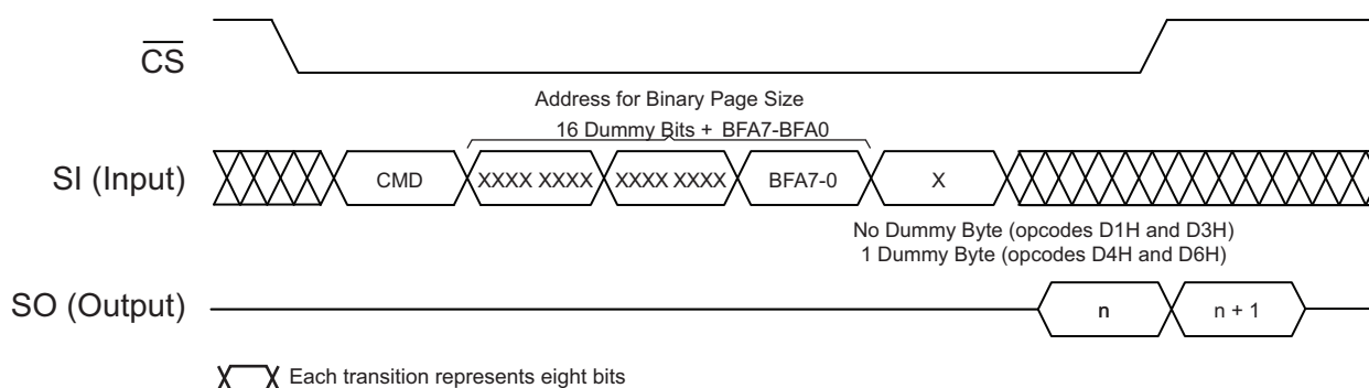
Figure 37. Buffer Read
