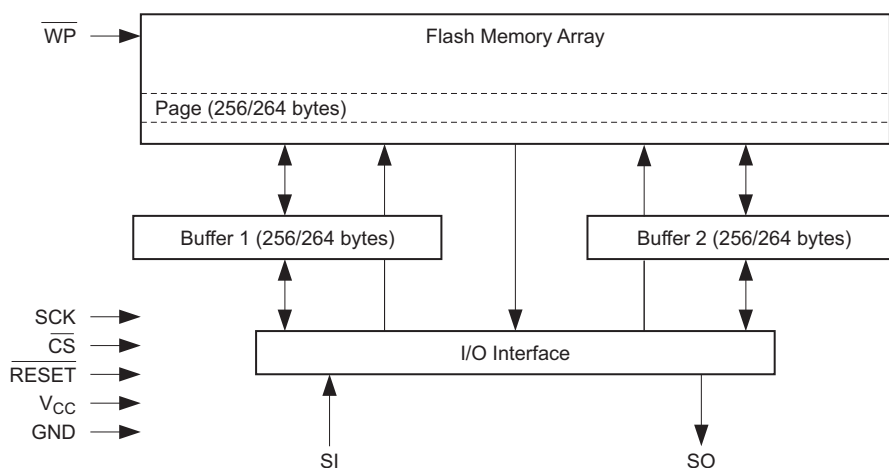
Figure 31. Block Diagram
