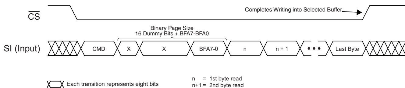
Figure 32. Buffer Write
