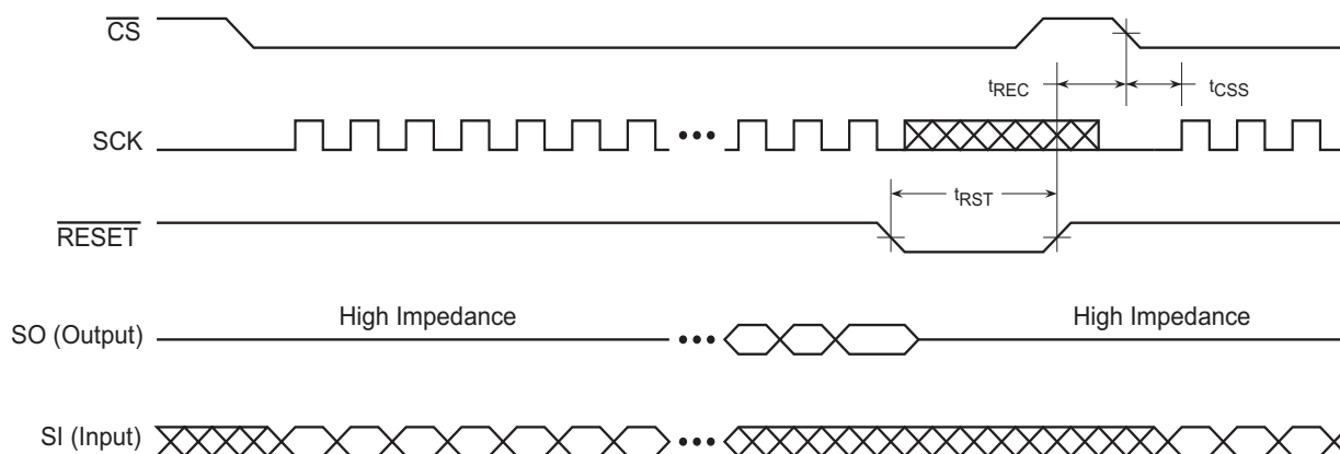
Figure 49. Reset Timing
