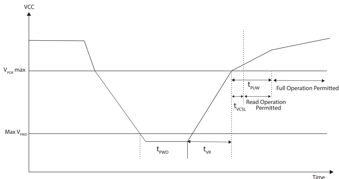
Figure 23. Power-Up Timing
