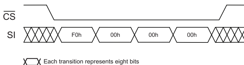
Figure 22. Software Reset
