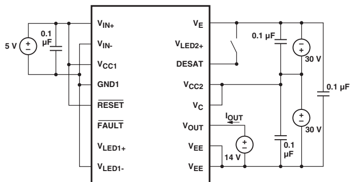
Figure 34. I_{OL} test circuit.
