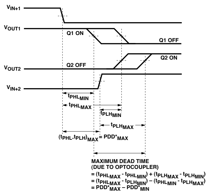
Figure 81. Waveforms for Dead Time Calculation.
