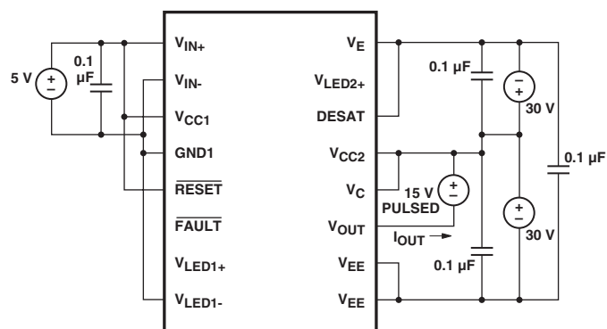
Figure 32. I_{OH} pulsed test circuit.
