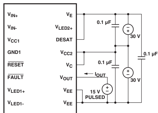
Figure 33. I_{OL} pulsed test circuit.
