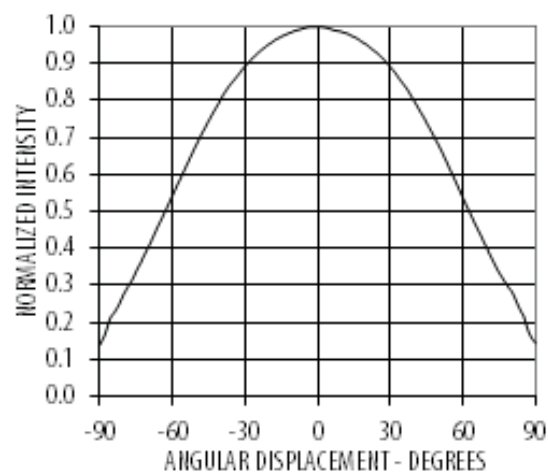
Figure 5 Radiation Pattern
