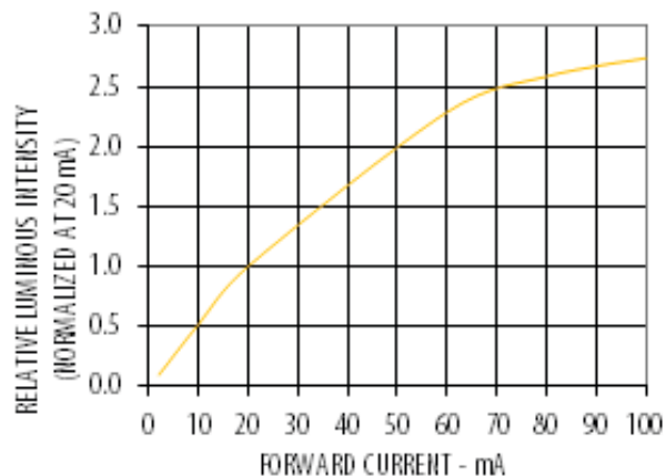
Figure 2 Relative Intensity vs. Forward Current
