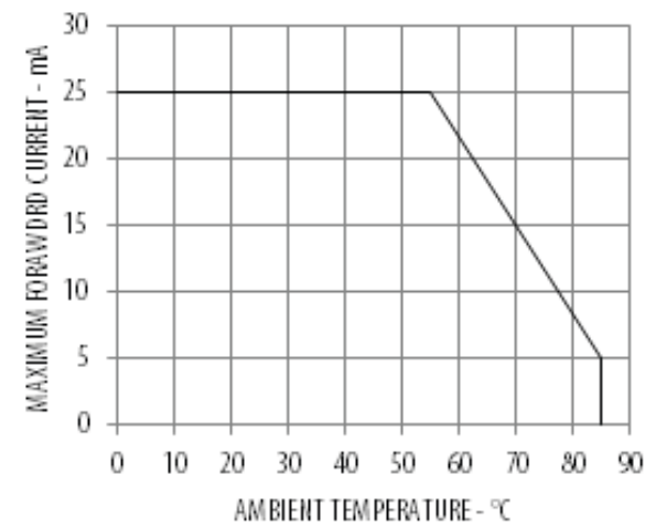
Figure 7 Derating Curve
