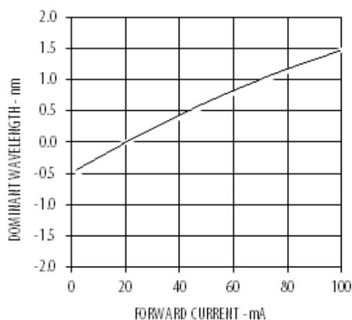
Figure 4 Dominant Wavelength Shift vs. Forward Current
