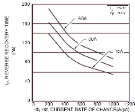
Figure 8. Reverse Recovery Time vs. Current Rate of Change
