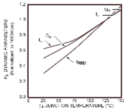
Figure 8. Dynamic Parameters vs. Junction Temperature
