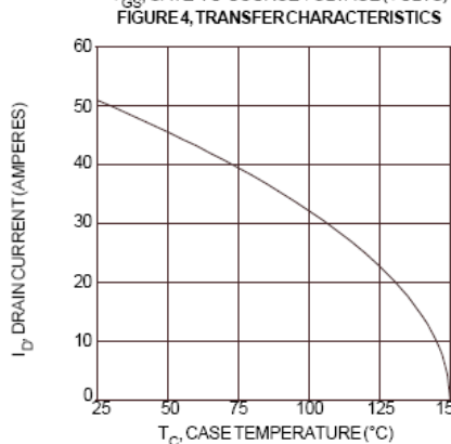
FIGURE 4, TRANSFER CHARACTERISTICS
