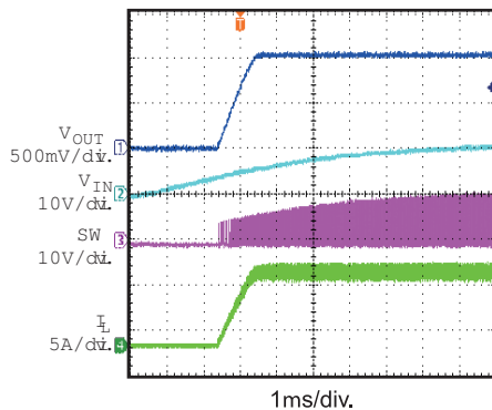
Start Up Through V_{IN} I_{OUT}=8A
