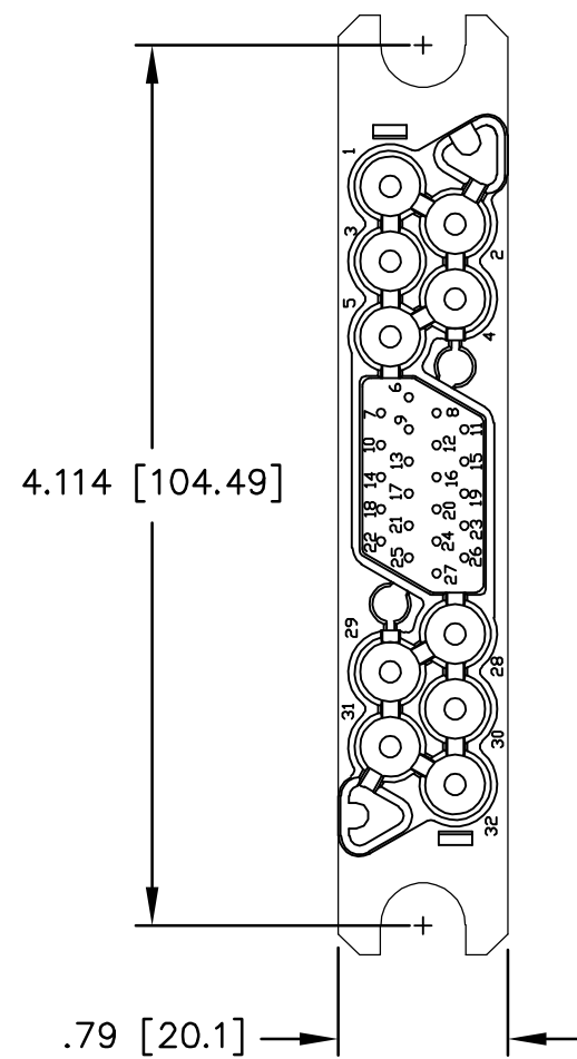
FRONT VIEW
