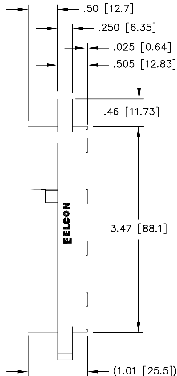
RIGHT SIDE
