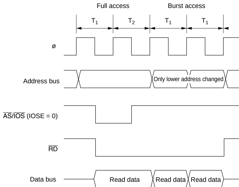
Figure 6.8 (b) Example of Burst ROM Access Timing (When AST = BRSTS1 = 0 )
