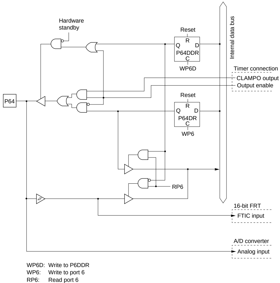
Figure C.20 Port 6 Block Diagram (Pin P64)
