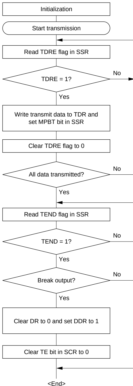
Figure 15.10 Sample Multiprocessor Serial Transmission Flowchart
