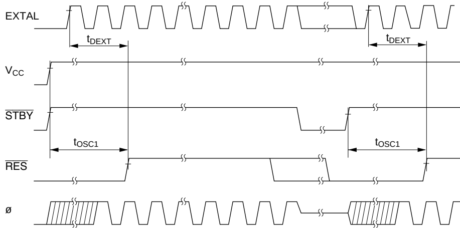
Figure 23.5 Oscillation Setting Timing
