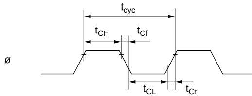
Figure 23.4 System Clock Timing
