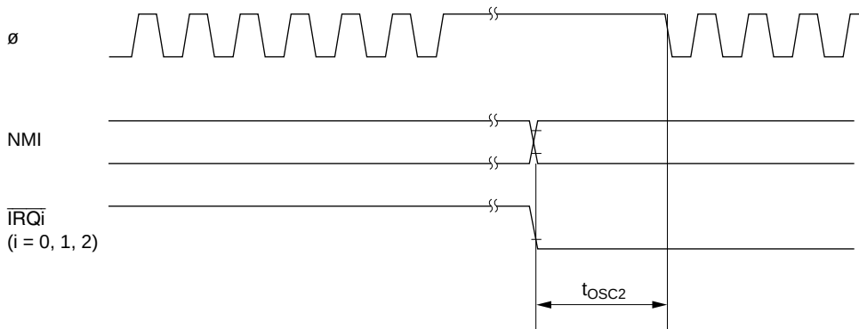
Figure 22.6 Oscillation Setting Timing (Exiting Software Standby Mode)
