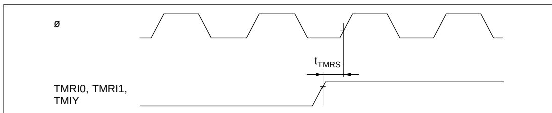
Figure 23.19 8-Bit Timer Reset Input Timing
