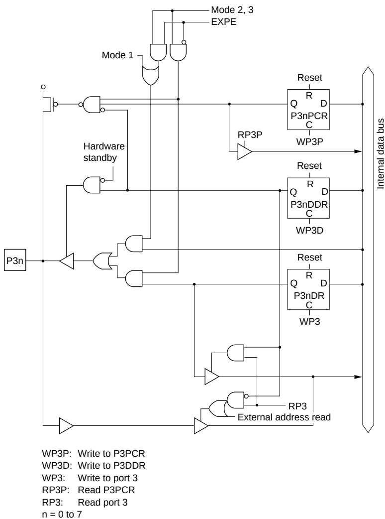
Figure C.9 Port 3 Block Diagram
