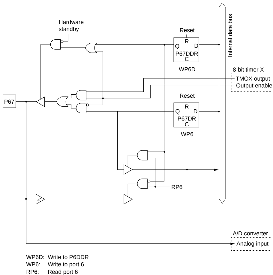
Figure C.22 Port 6 Block Diagram (Pin P67)
