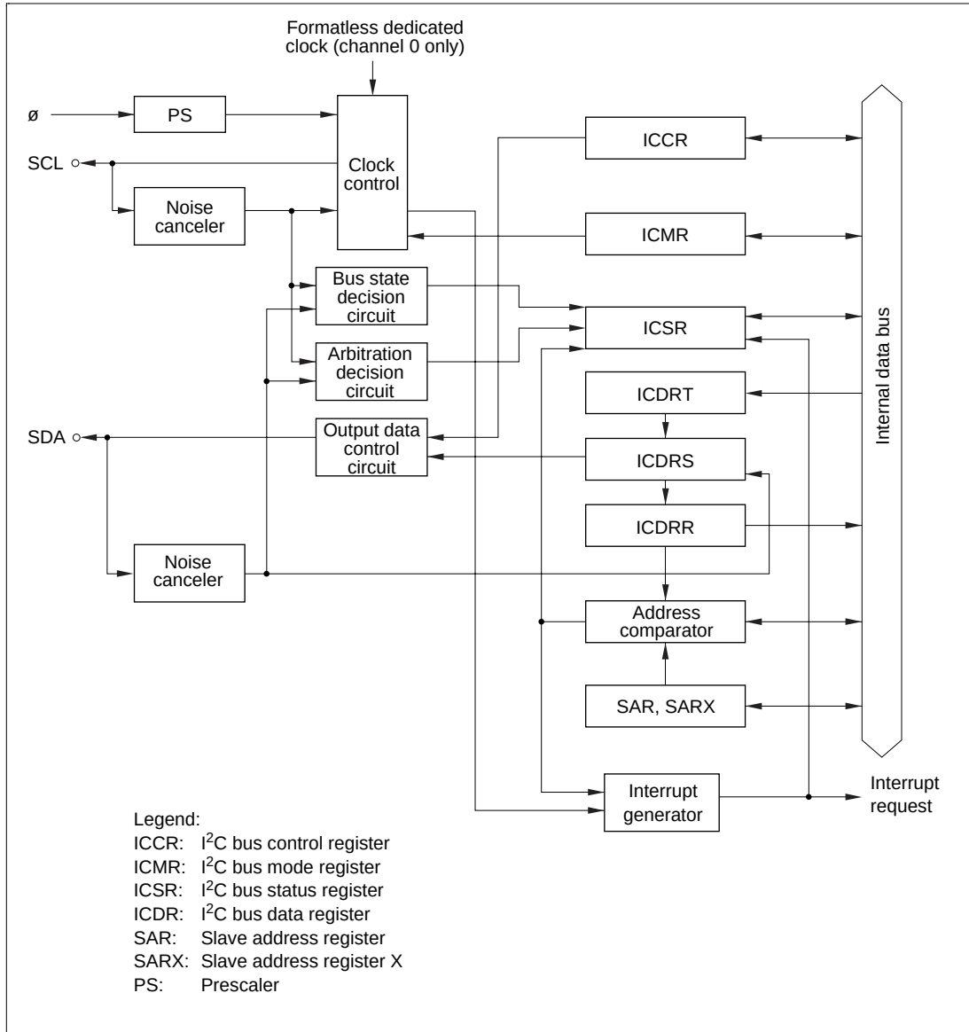
Figure 16.1 Block Diagram of I²C Bus Interface
