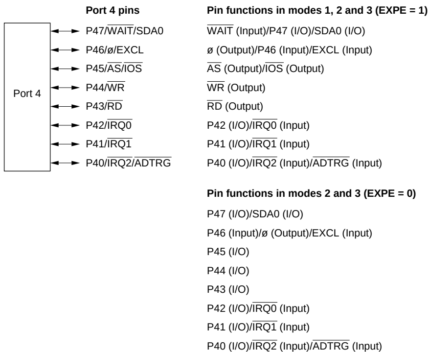
Figure 8.12 Port 4 Pin Functions
