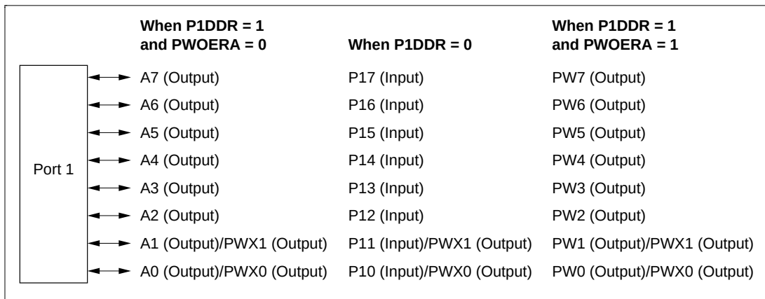
Figure 8.3 Port 1 Pin Functions (Modes 2 and 3 (EXPE = 1))
