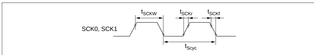
Figure 23.20 SCK Clock Input Timing
