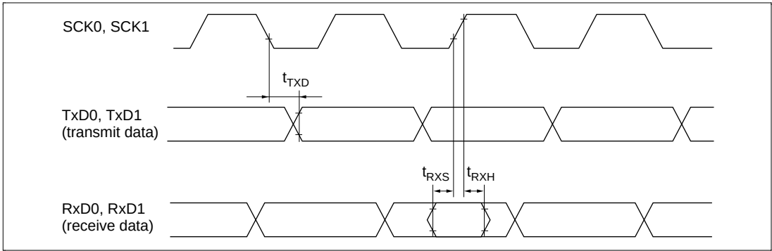
Figure 23.21 SCI Input/Output Timing (Synchronous Mode)
