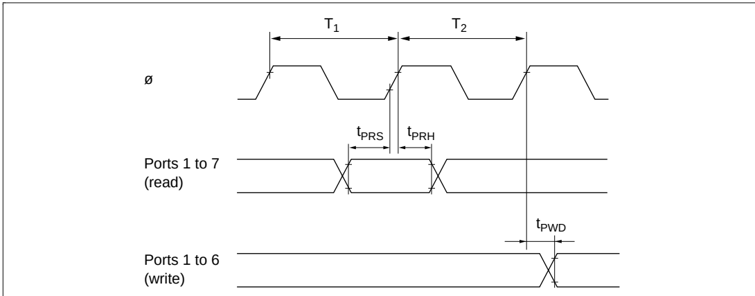
Figure 23.14 I/O Port Input/Output Timing
