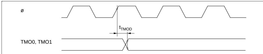
Figure 23.17 8-Bit Timer Output Timing
