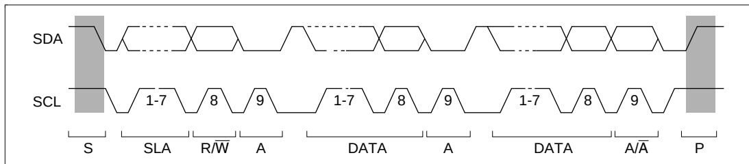
Figure 16.6 I²C Bus Timing
