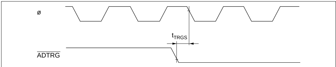
Figure 23.22 A/D Converter External Trigger Input Timing
