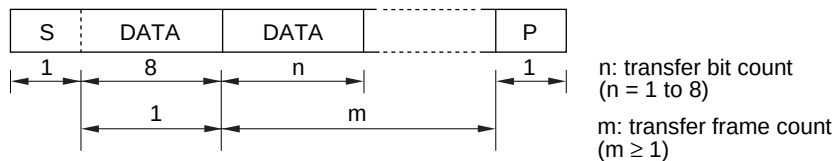
Figure 16.5 I²C Bus Data Format (Serial Format)
