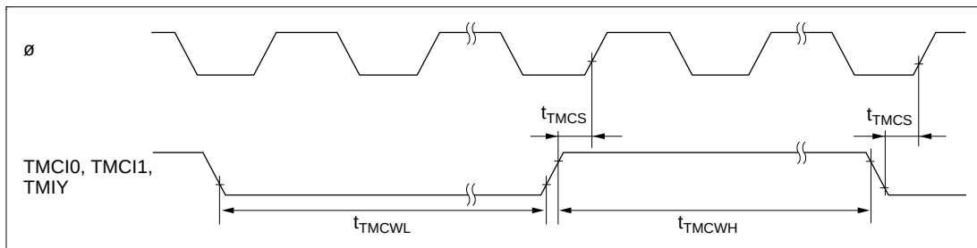
Figure 23.18 8-Bit Timer Clock Input Timing
