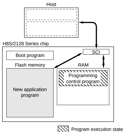
Figure 19.4 Boot Mode
