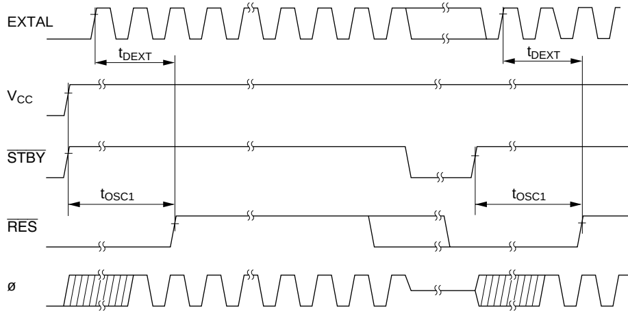
Figure 22.5 Oscillation Setting Timing
