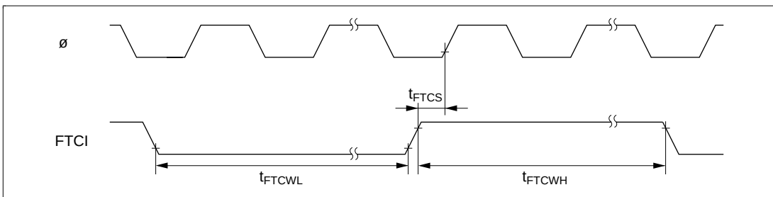
Figure 23.16 FRT Clock Input Timing
