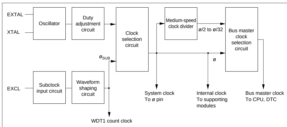
Figure 20.1 Block Diagram of Clock Pulse Generator
