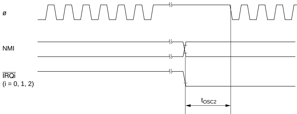
Figure 23.6 Oscillation Setting Timing (Exiting Software Standby Mode)
