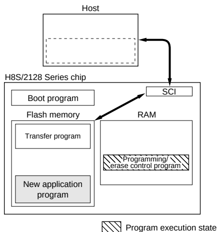
Figure 19.5 User Program Mode (Example)
