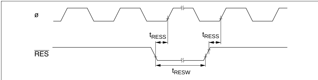
Figure 23.7 Reset Input Timing
