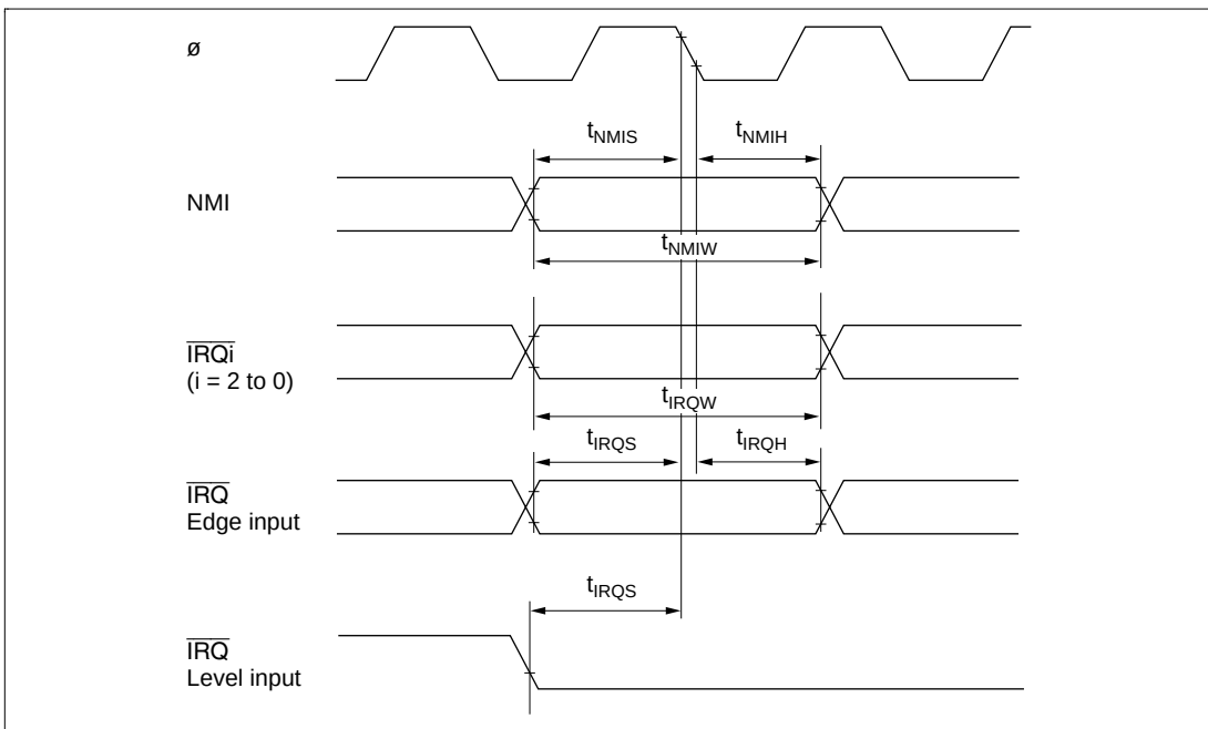
Figure 23.8 Interrupt Input Timing
