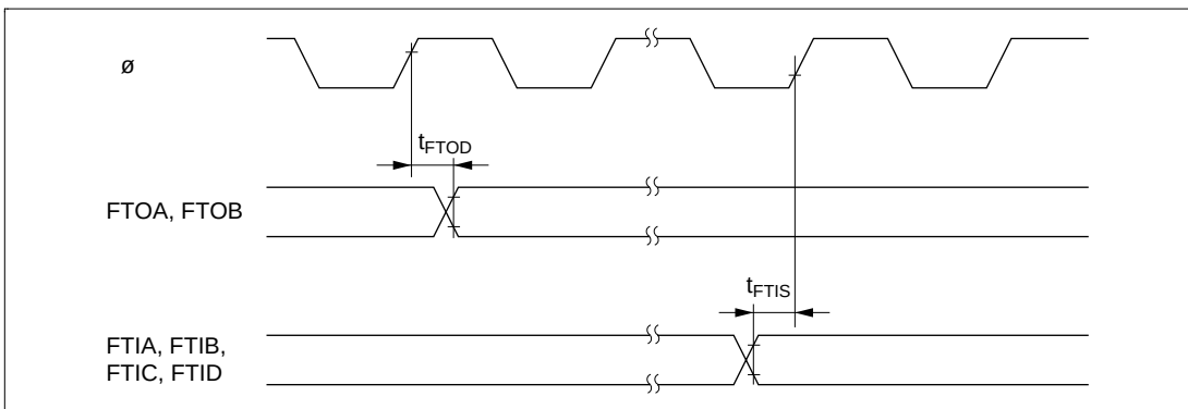
Figure 23.15 FRT Input/Output Timing
