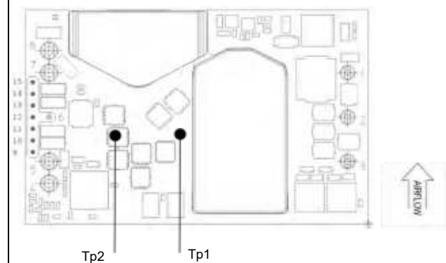
Base plate (Bottom view)
