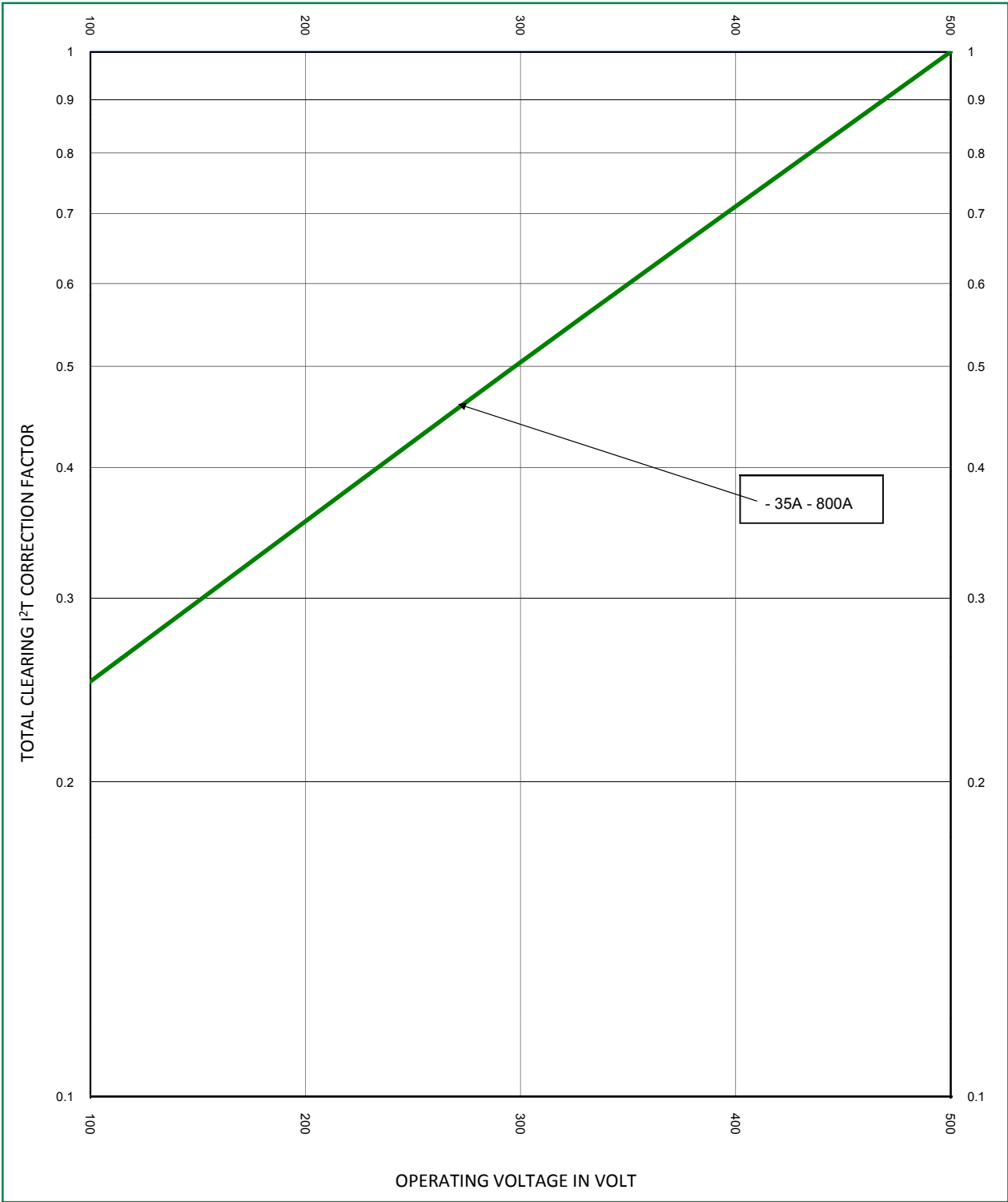
Total Clearing I²t Correction Factor Curve L50QS Series
