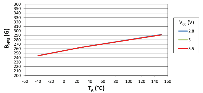
Average Switchpoint Hysteresis versus Ambient Temperature
