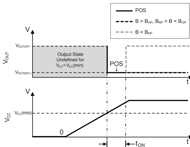
Figure 2: Power-On Timing Diagram
