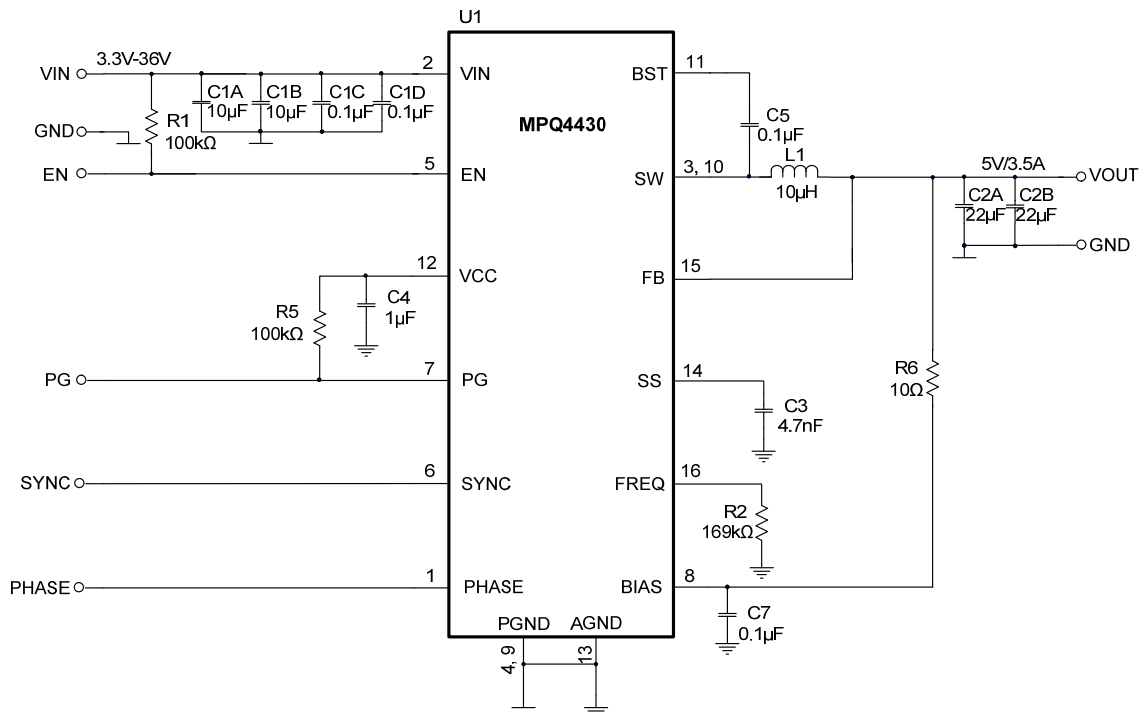
Figure 18: 5V Fixed Output, F SW = 500kHz
