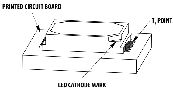
Figure 23: Solder Point Temperature on PCB
