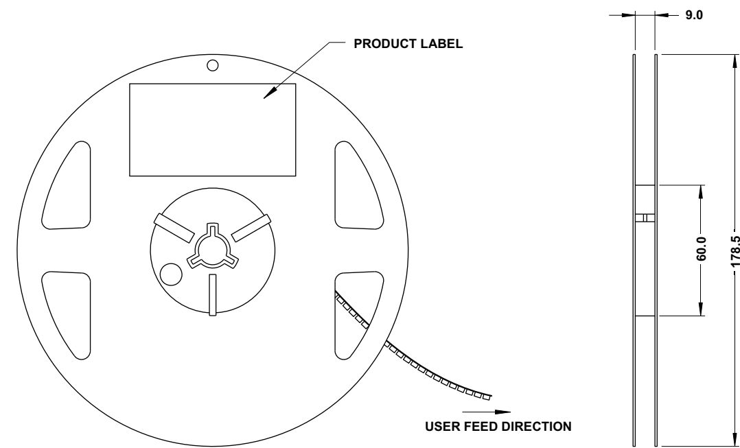
Figure 20: Reel Dimension
