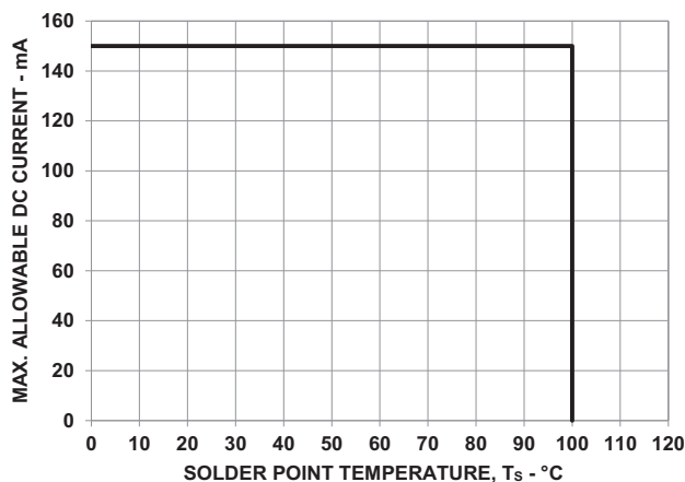
Figure 16: Maximum Forward Current vs. Solder Point Temperature. Derated Based on T_{JMAX} = 125^{\circ}C , R_{\theta JS} = 40^{\circ}C/W .
