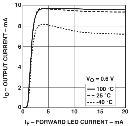
Figure 11: Typical Transfer Characteristics
