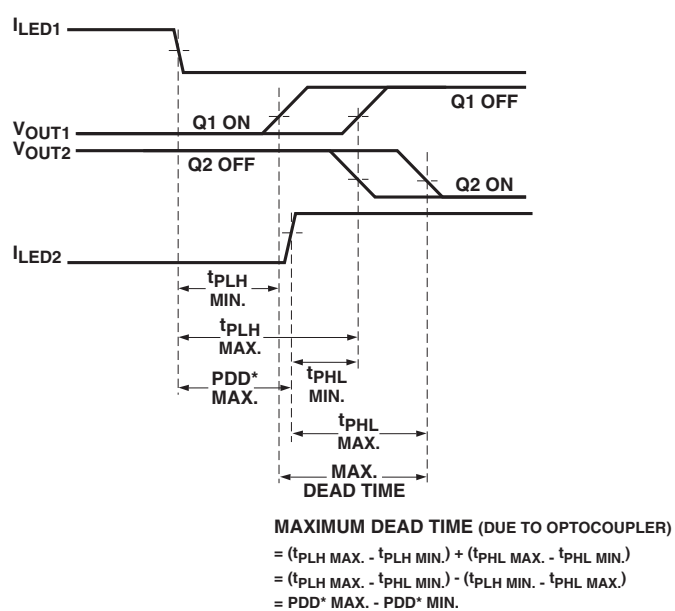
Figure 37: Waveforms for Dead Time Calculation
