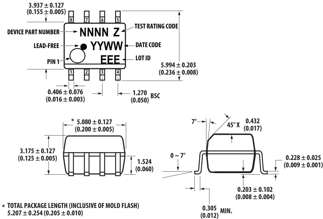
Figure 6: HCPL-0466 Outline Drawing (8-Pin Small Outline Package)
