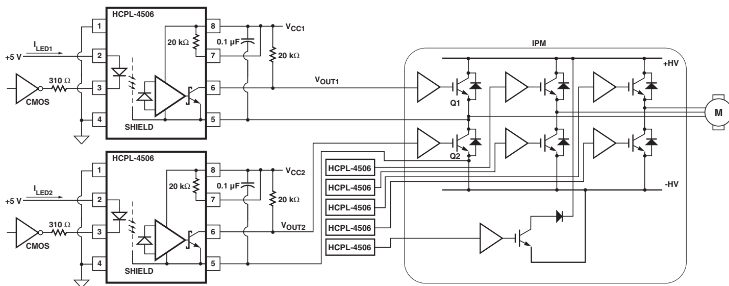
Figure 35: Typical Application Circuit
