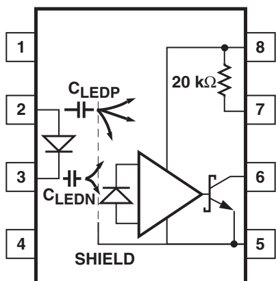
Figure 27: Optocoupler Input-to-Output Capacitance Model for Unshielded Optocouplers
