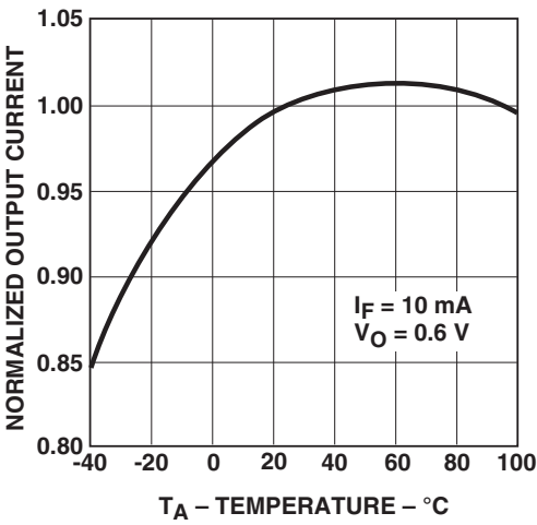
Figure 12: Normalized Output Current vs. Temperature
