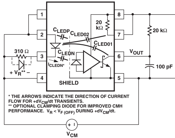
Figure 31: AC Equivalent Circuit for Figure 26 during Common Mode Transients
