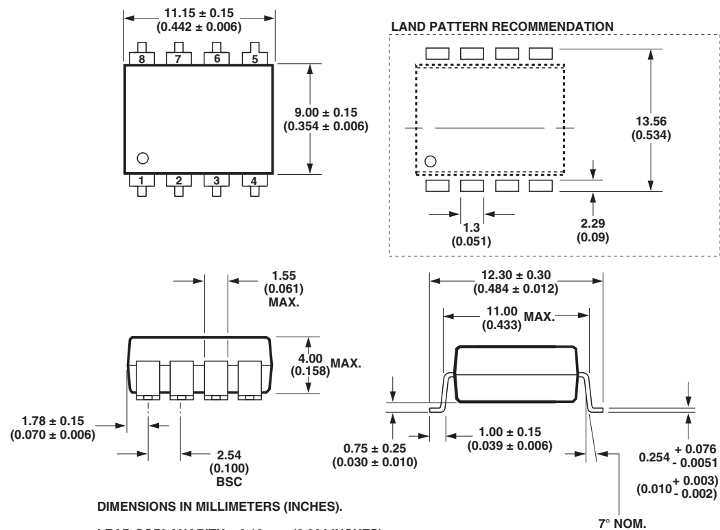
Figure 8: HCNW4506 Gull Wing Surface-Mount Option 300 Outline Drawing
