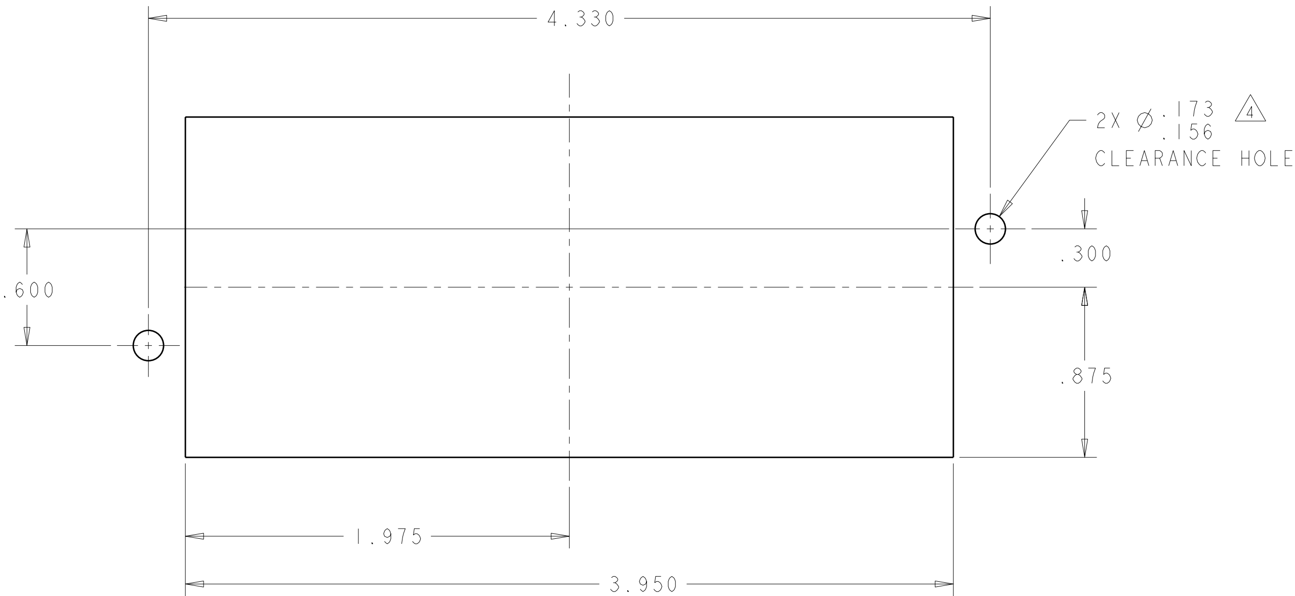
PANEL CUT-OUT COMPONENT SIDE
