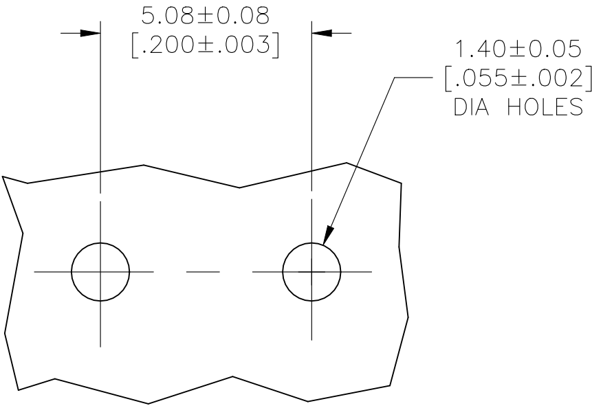
P.C. BOARD HOLE PATTERN
