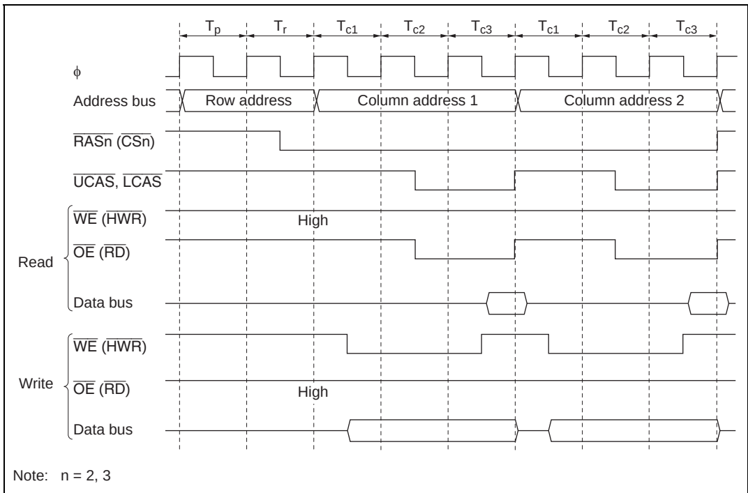
Figure 6.30 Operation Timing in Fast Page Mode (RAST = 0, CAST = 1)
