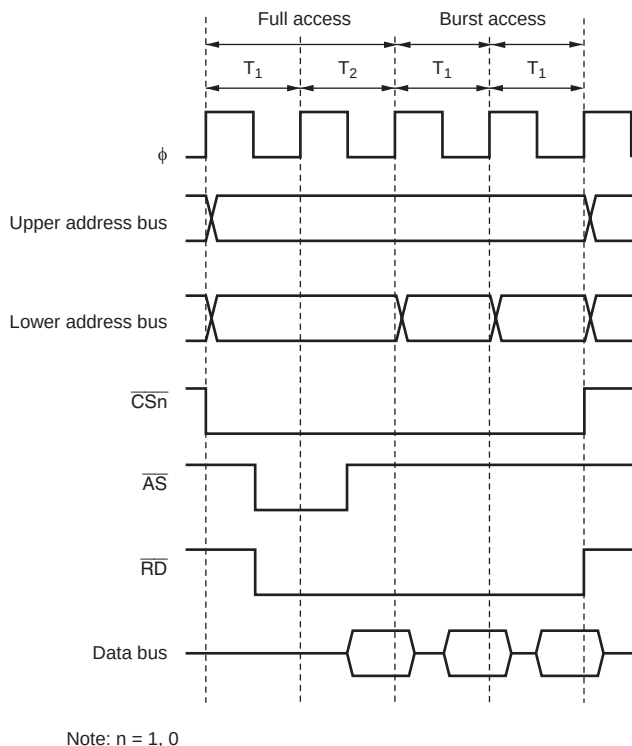
Figure 6.43 Example of Burst ROM Access Timing (ASTn = 0, 1-State Burst Cycle)
