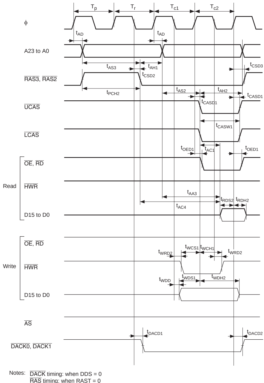
Figure 25.13 DRAM Access Timing: Two-State Access
