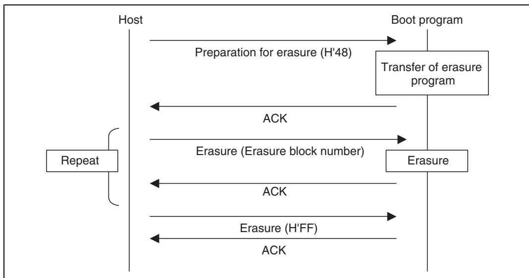
Figure 20.22 Erasure Sequence
