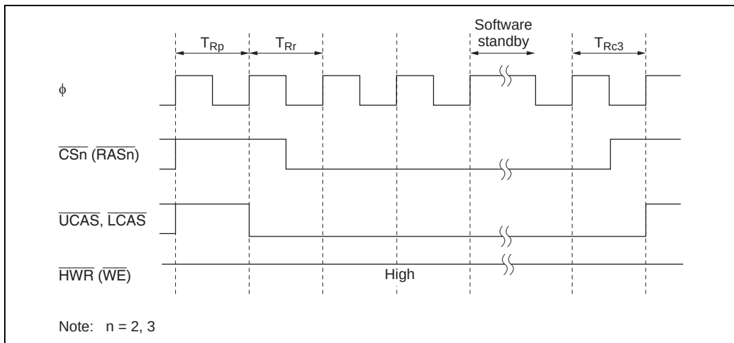
Figure 6.38 Self-Refresh Timing
