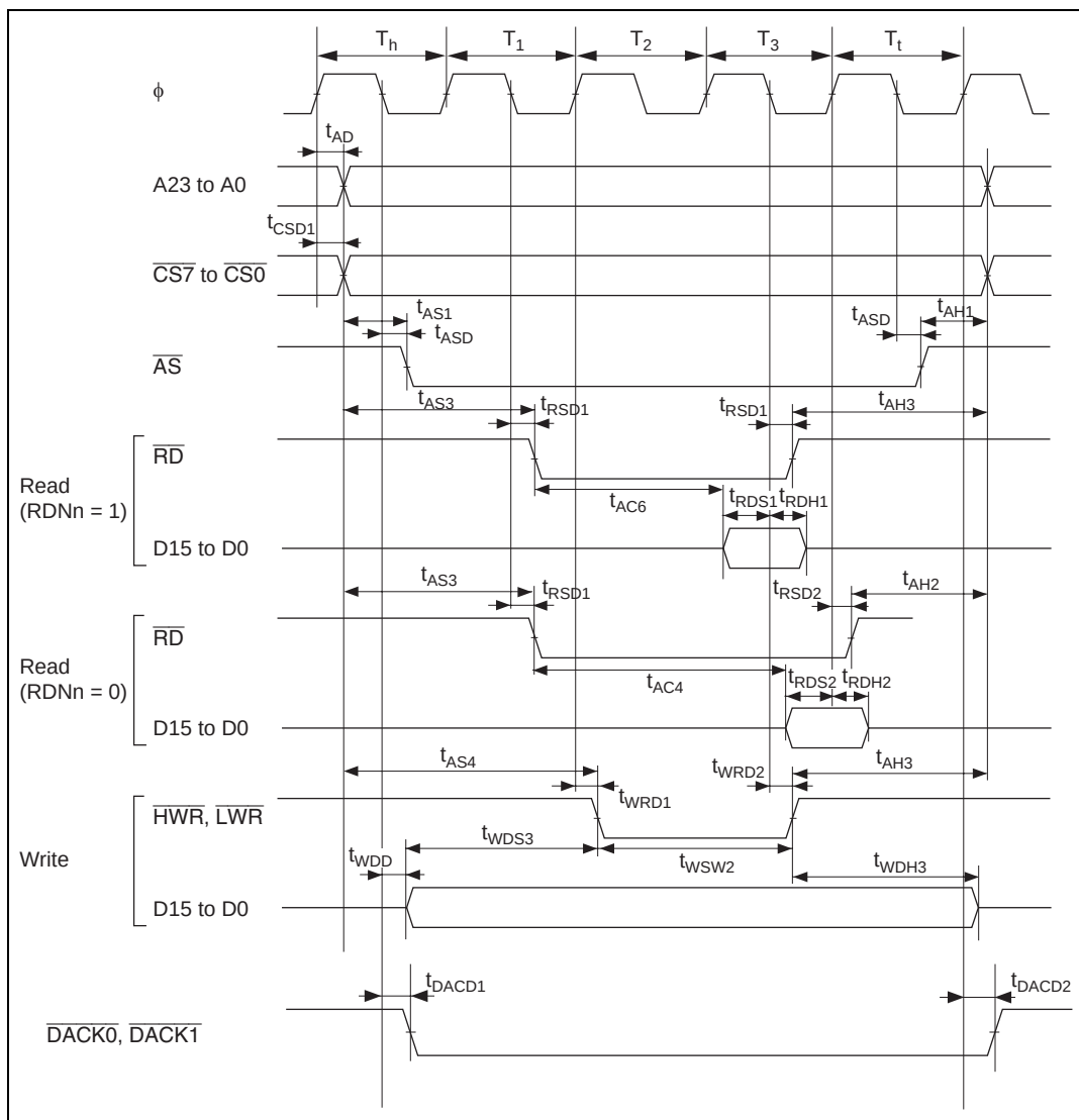
Figure 25.10 Basic Bus Timing: Three-State Access ( \overline{\text{CS}} Assertion Period Extended)
