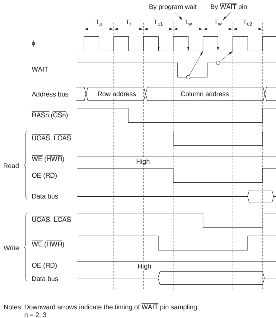
Figure 6.25 Example of Wait State Insertion Timing (2-State Column Address Output)
