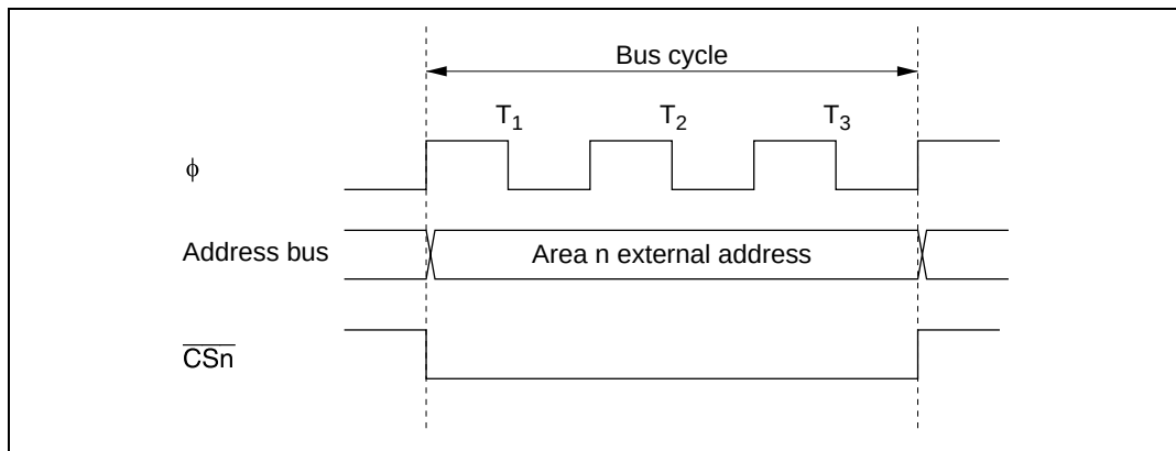
Figure 6.6 \overline{\text{CSn}} Signal Output Timing ( n = 0 to 7)
