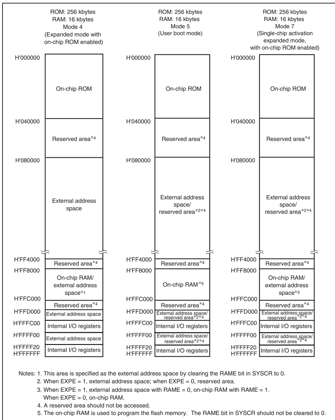
Figure 3.12 H8S/2360F Memory Map (2)
