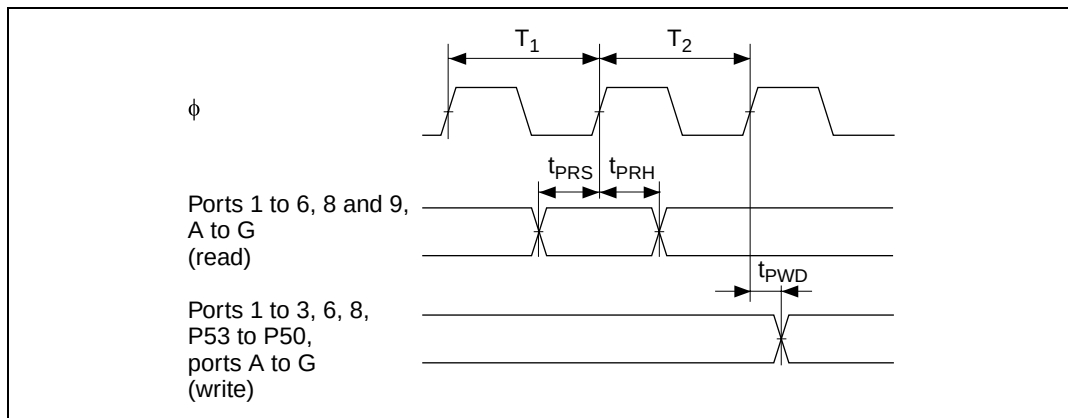
Figure 25.28 I/O Port Input/Output Timing
