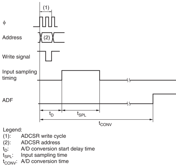
Figure 16.2 A/D Conversion Timing
