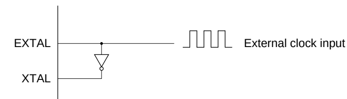
(b) Counter clock input at XTAL pin
