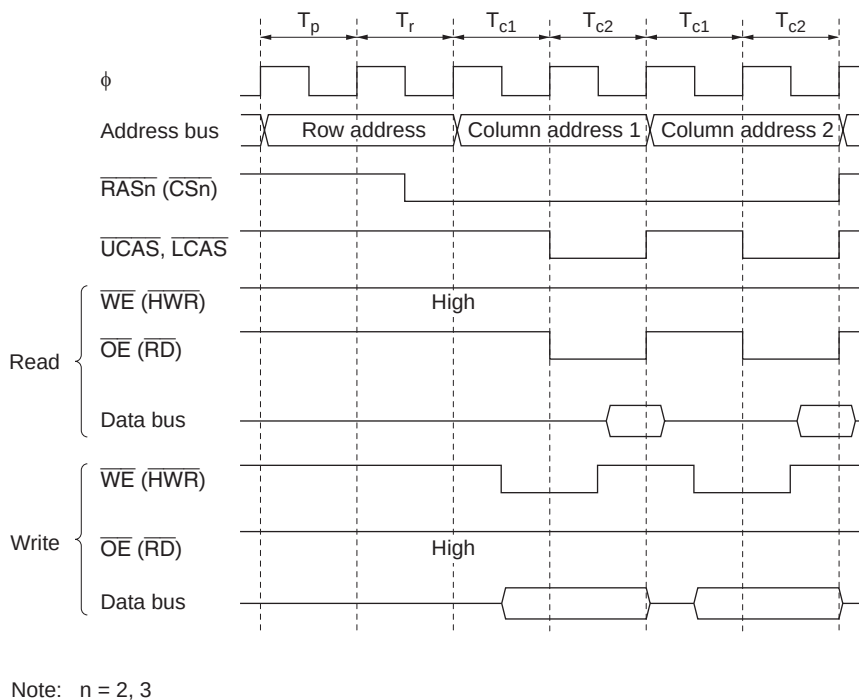
Figure 6.29 Operation Timing in Fast Page Mode (RAST = 0, CAST = 0)
