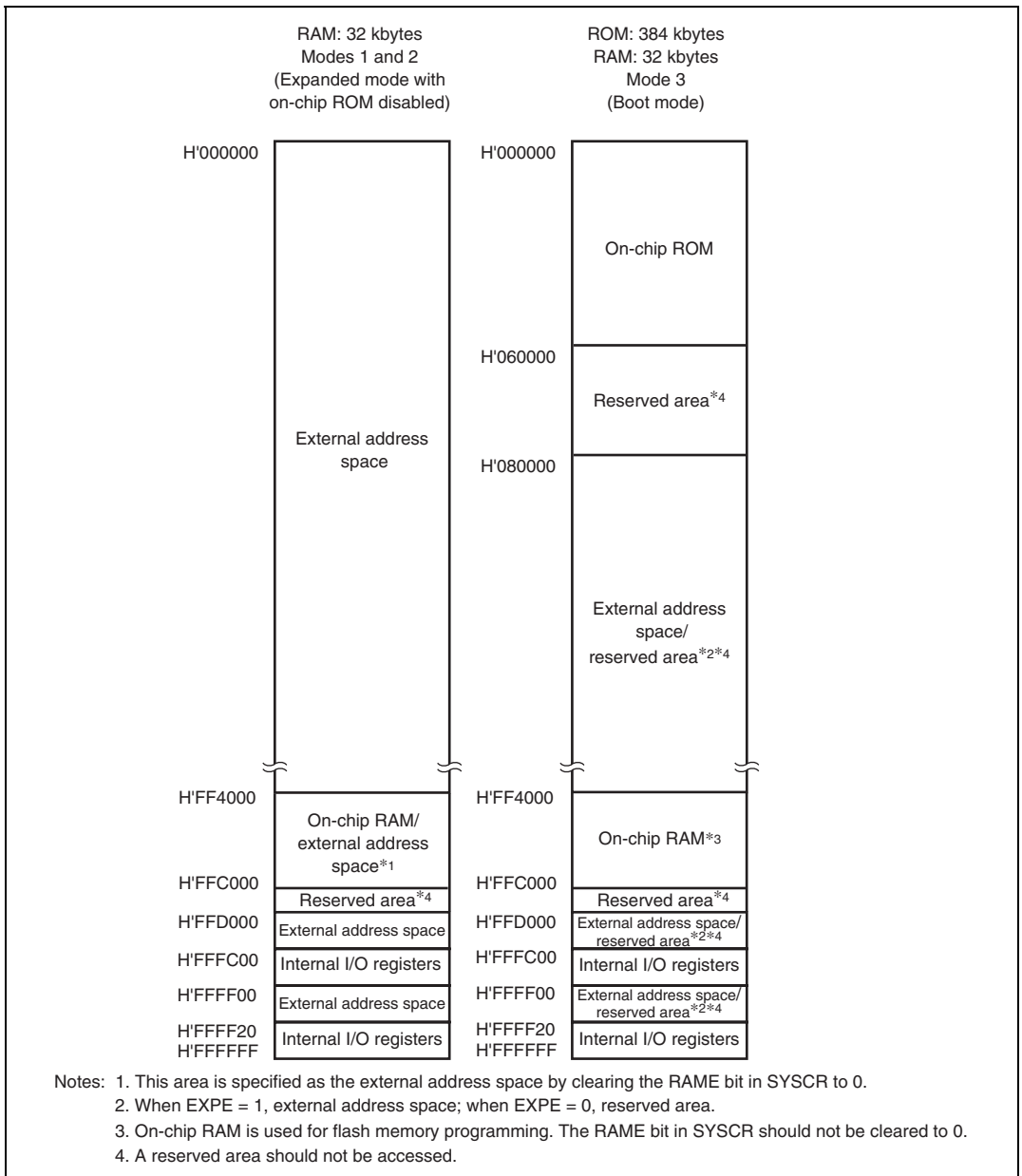
Figure 3.5 H8S/2364F Memory Map (1)
