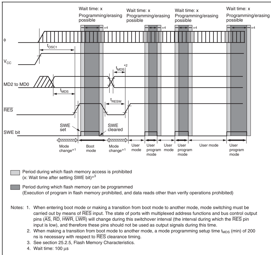
Figure 19.10 Mode Transition Timing (Example: Boot Mode → User Mode ↔ User Program Mode)
