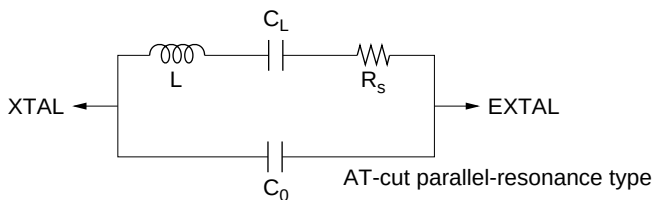
Figure 22.3 Crystal Oscillator Equivalent Circuit
