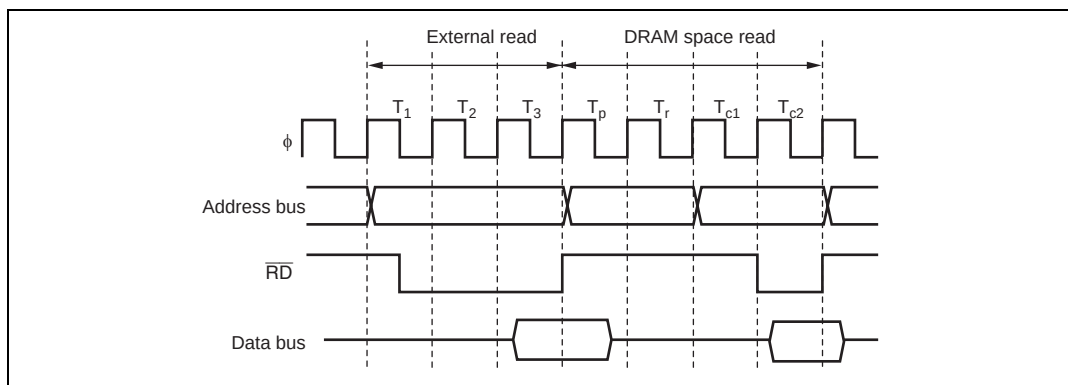
Figure 6.48 Example of DRAM Full Access after External Read (CAST = 0)
