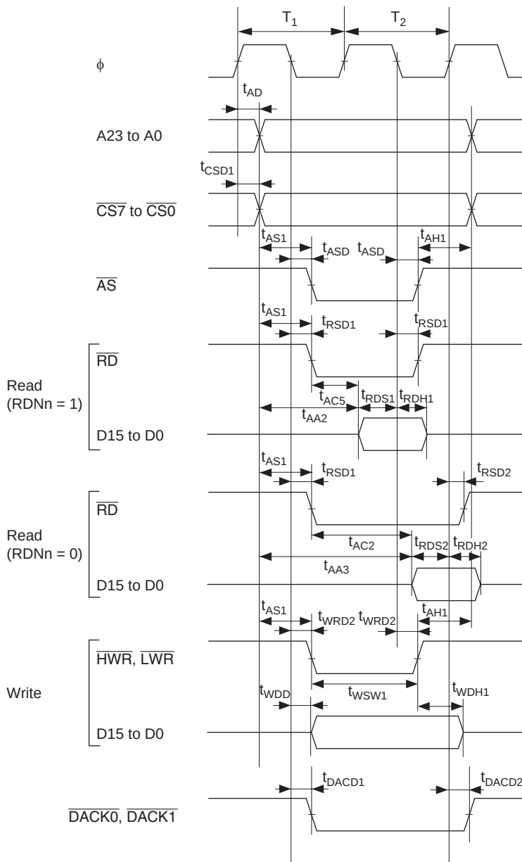
Figure 25.6 Basic Bus Timing: Two-State Access
