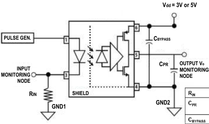
Figure 10: Switching Speed Test Circuit and Typical Waveform
