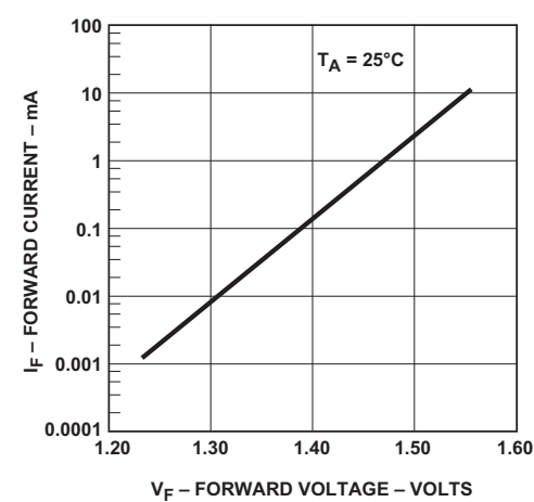
Figure 10: LED Input Current vs. Forward Voltage
