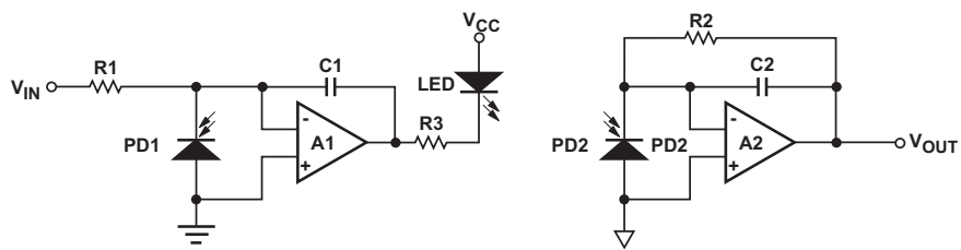
B) PRACTICAL CIRCUIT
