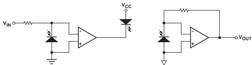
A) POSITIVE INPUT
