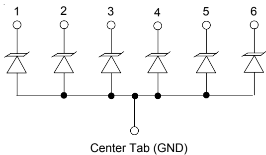
Device Schematic
