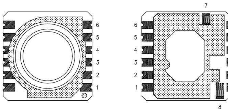
Fig. 2: Pin configuration of MS5534C
