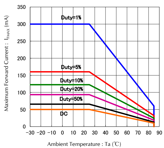
Ambient Temperature vs. Maximum Forward Current Condition : t_w \leq 0.1\text{ms}
