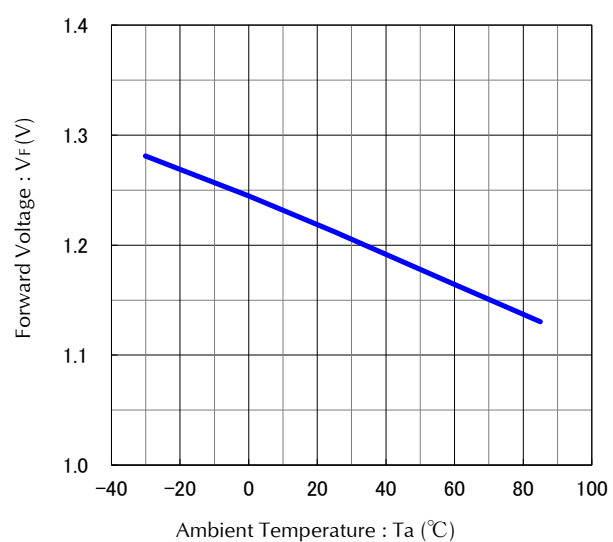
Ambient Temperature vs. Forward Voltage Condition : I_F = 20\text{mA}
