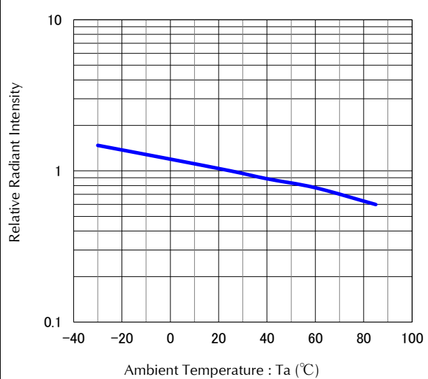
Ambient Temp. vs. Relative Radiant Intensity Condition : I_F = 20\text{mA}
