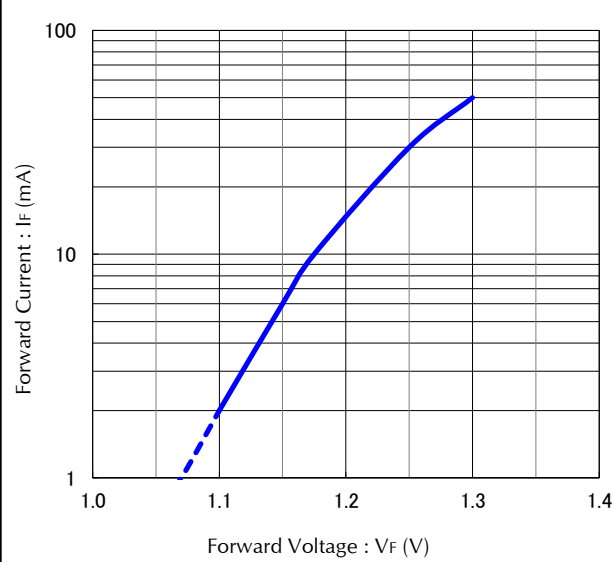
Forward Voltage vs. Forward Current Condition : T_a = 25^\circ\text{C}
