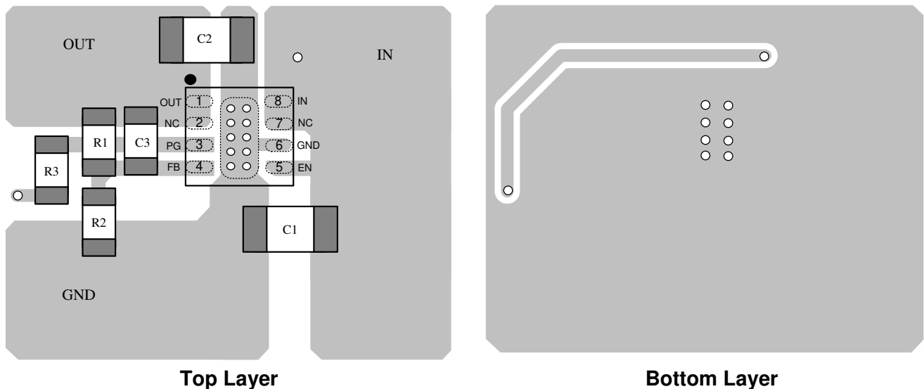
Figure 2—PCB Layout
