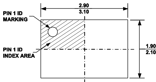
QFN8 (2mm x 3mm)
