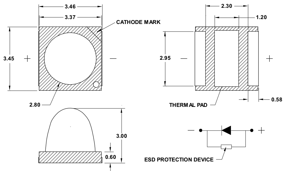
Figure 2: Package Drawing for AUV4-SxD1-0xx0J
