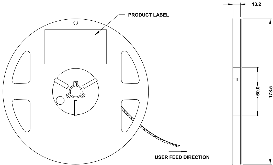
Figure 19: Reel Dimensions
