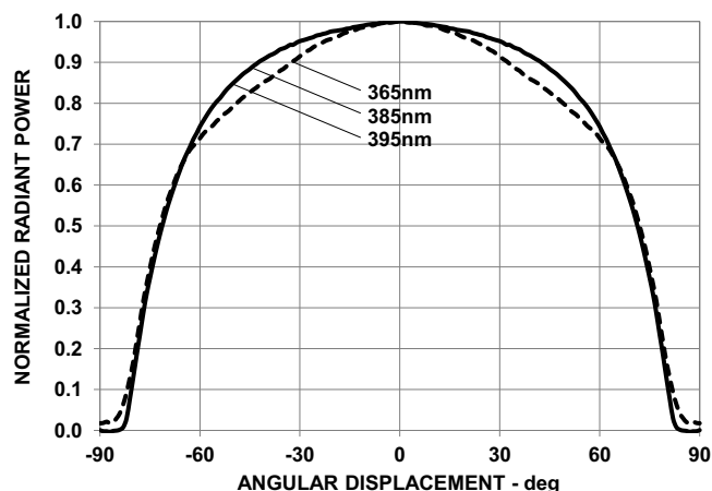
Figure 10: Radiation Pattern – 130°
