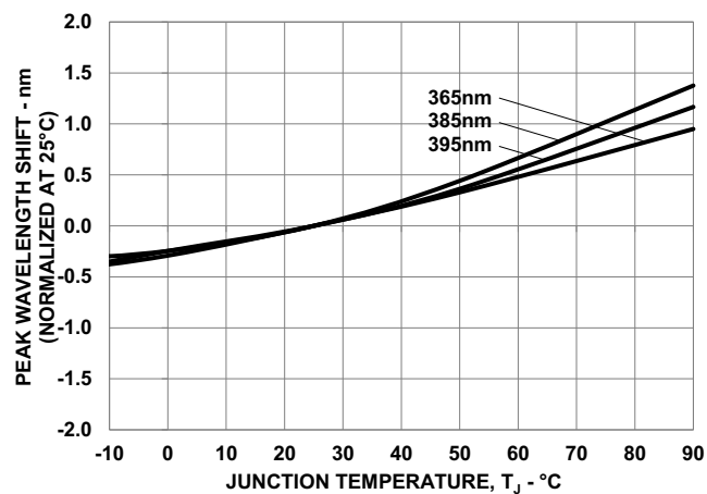
Figure 12: Peak Wavelength Shift vs. Junction Temperature
