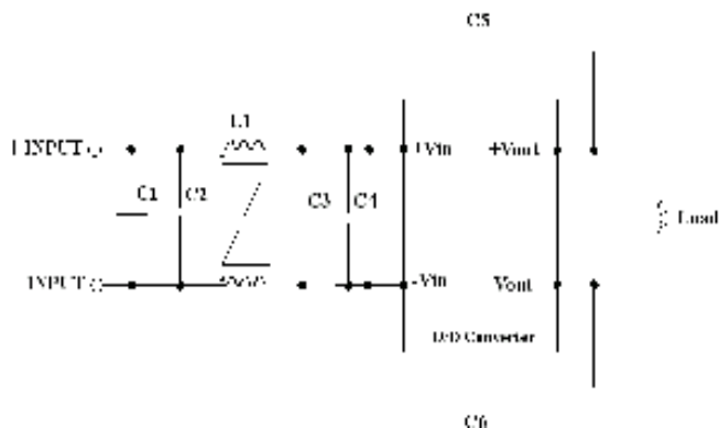
Suggested Schematic for EN55022 Conducted Emissions Class B Limits
