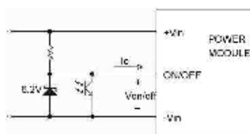
Level Control Using Line Voltage
