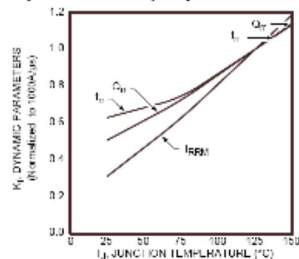
Figure 8. Dynamic Parameters vs. Junction Temperature
