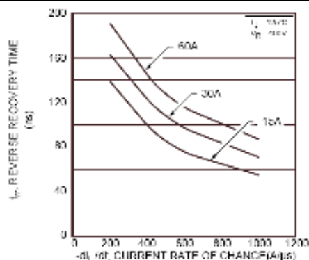
Figure 8. Reverse Recovery Time vs. Current Rate of Change
