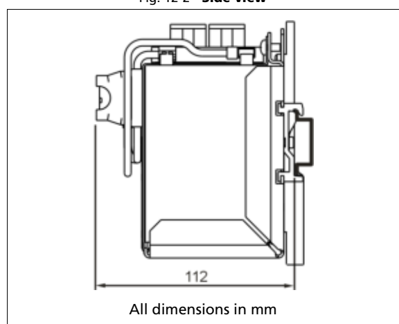
Fig. 12-2 Side view
