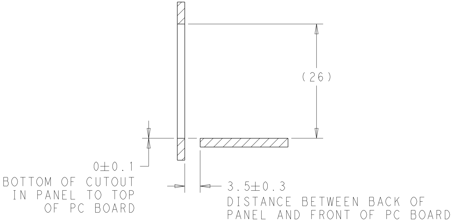
SECTION U-U
