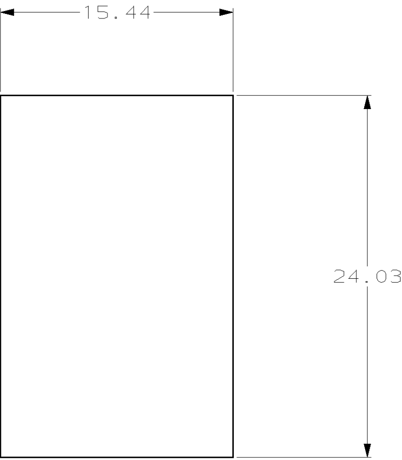
RECOMMENDED CUT OUT FOR 1.57 MAX THICK PANEL
