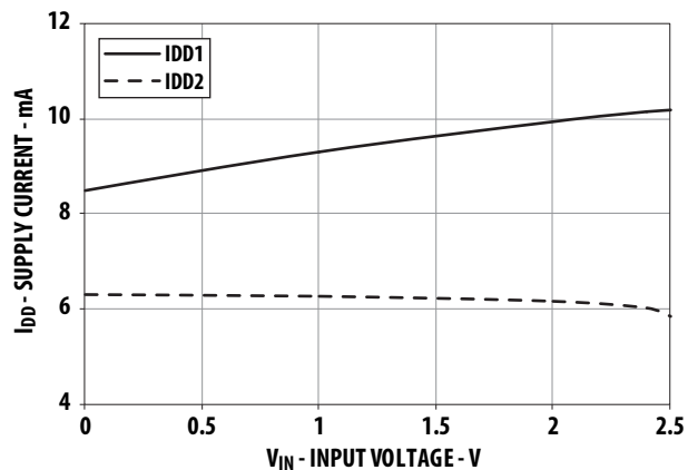
Figure 18: Typical Supply Current vs. Input Voltage
