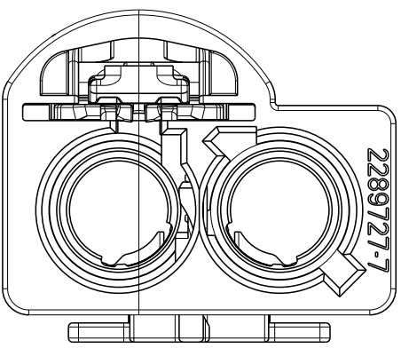
DETAIL G SCALE 3:1
