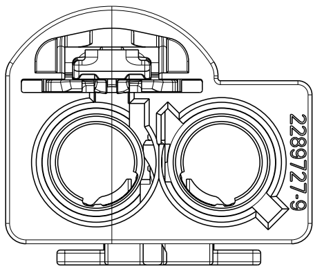
DETAIL I SCALE 3:1
