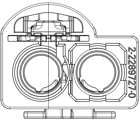
DETAIL N SCALE 3:1
