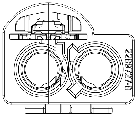
DETAIL H SCALE 3:1
