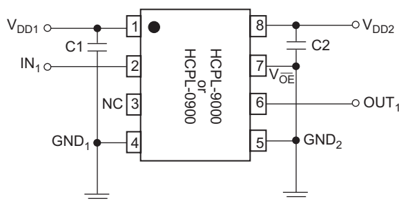
Figure 1: Functional Diagram of Single-Channel HCPL-0900 or HCPL-0900
