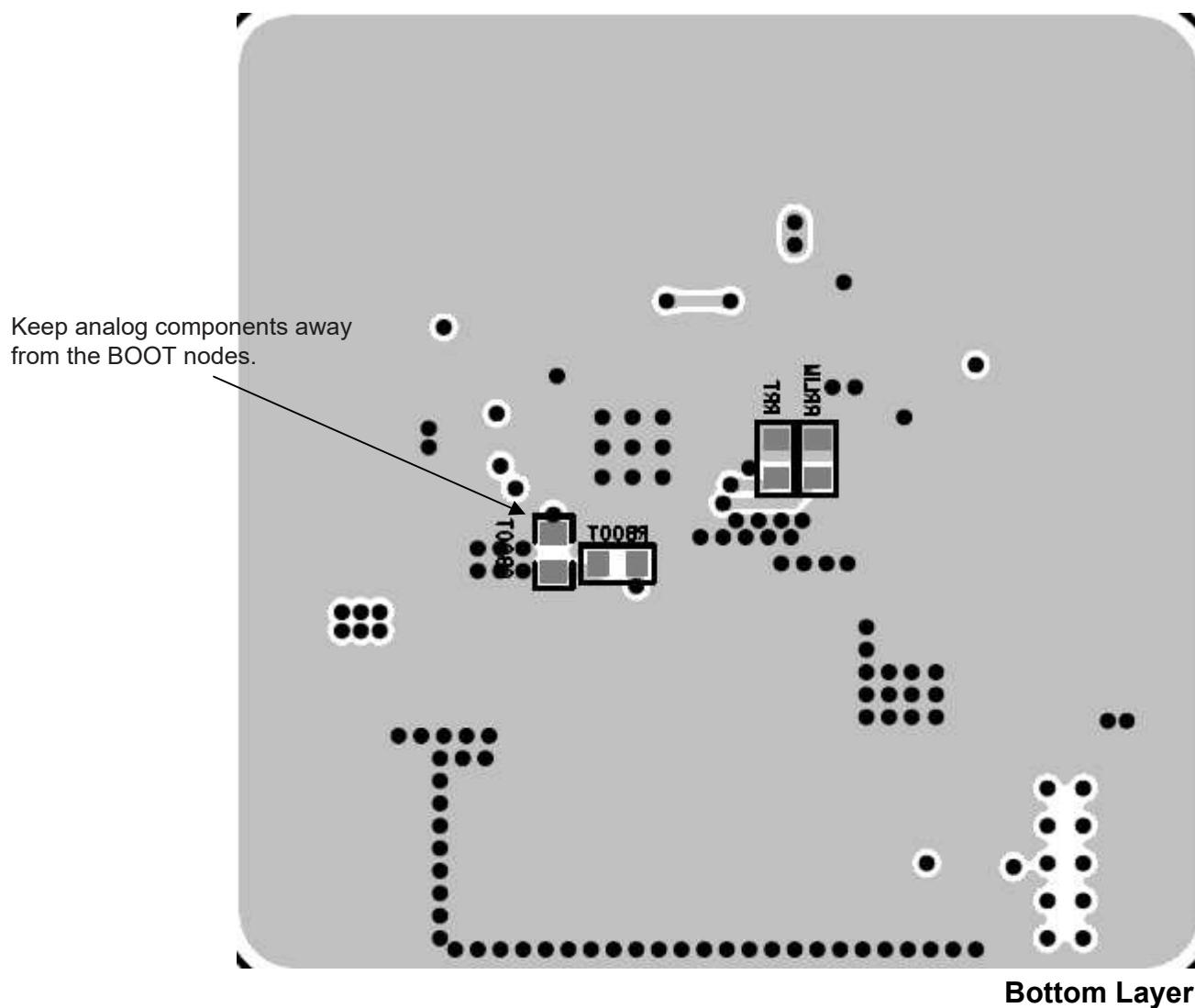
Figure 27. Layout Guide (Bottom Layer)
