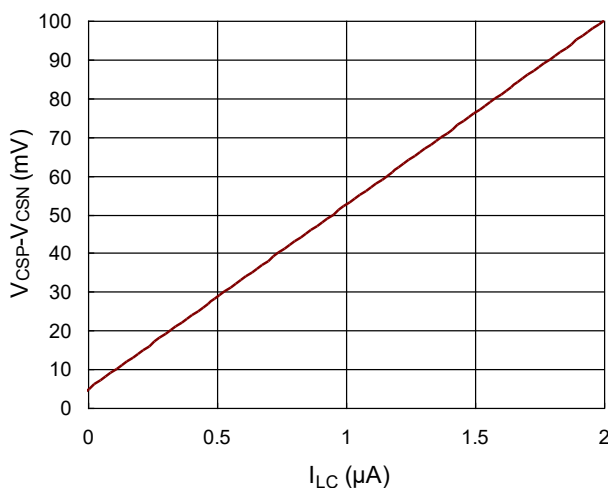
Figure 21. I_{LC} vs. V_{CSP} - V_{CSN}
