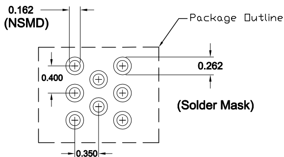
RECOMMENDED LAND PATTERN (PCB Top view, NSMD Design)
