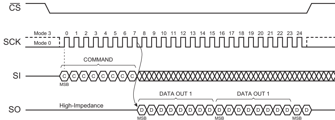
Figure 5. SPI Transfer — Command and Data Only — Read Operation
