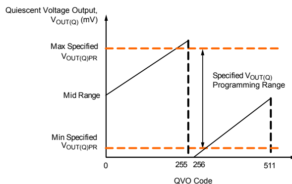
Figure 8: Device V_{OUT(Q)} versus QVO Programmed Value
