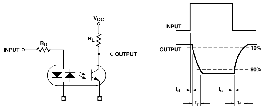
Figure 12. Test circuit for response time.
