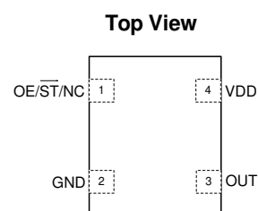
Figure 1. Pin Assignments
