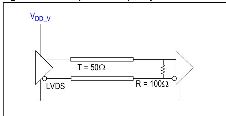
Figure 12. LVDS (STYLE = 0) Output Termination
