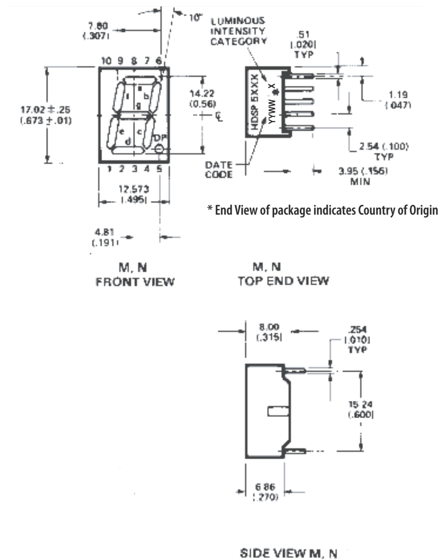
Figure 4: Package Dimensions, M to N
