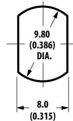
Figure 2. Recommended cut-out for panel mounting
